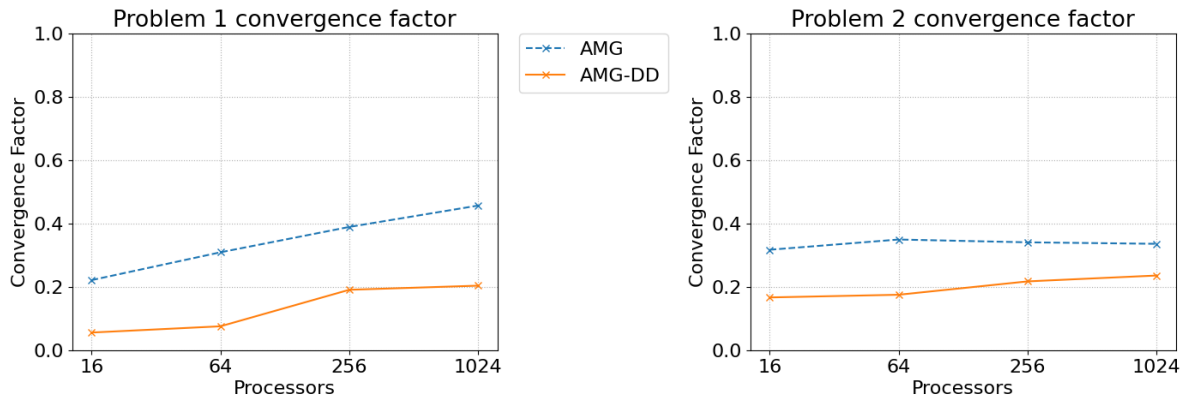
FIGURE 17 Convergence factor weak scaling for AMG vs. AMG-DD wrapped with BiCGSTAB for 3D Poisson (left) and rotated anisotropic diffusion (right).
