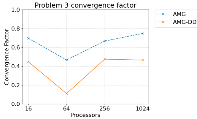
FIGURE 19 Convergence factor weak scaling for AMG vs. AMG-DD wrapped with BiCGSTAB on Problem 3 with multiple difficulties.
