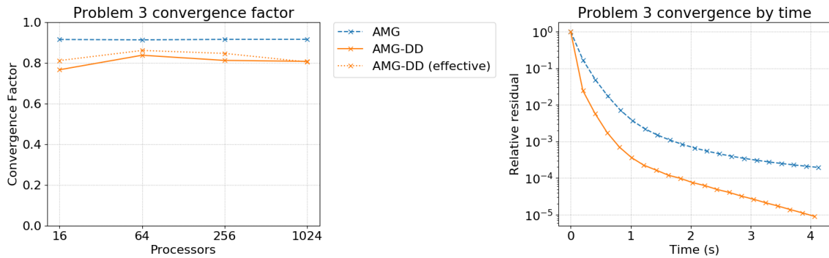
FIGURE 18 Asymptotic convergence factors for different processor counts (left) and convergence by time with 1,024 processors (right) for AMG vs. AMG-DD on Problem 3 with multiple difficulties.
