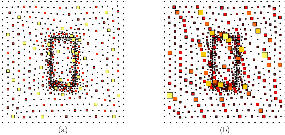
FIG. 4.4. Grid hierarchies produced by CR-AMG (a) and BoomerAMG (b) for the rotated anisotropic problem 2D-M2-RLap. Larger squares depict grid points on coarser-level grids.
