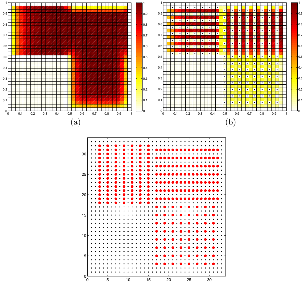
FIG. 4.1. Candidate measures \gamma_i computed at step 3.1d during stage one (a) and two (b) for problem 2D-4Reg-Q. Each square depicts the value of \gamma_i at grid point i according to the color bar. Dotted squares indicate points currently in C ( C -points). The final coarse grid is given by the larger red circles in (c).
